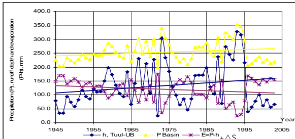
Fig. 5 Annual runoff /hmm/, basin average precipitation /P basin / and evapotranspiration or evapotranspiration and change in water storage /E±ΔS/
