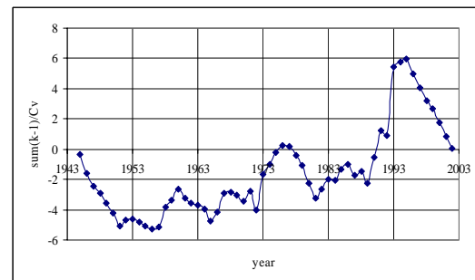
Fig. 3 Cyclic pattern of annual flows of the Tuul river
