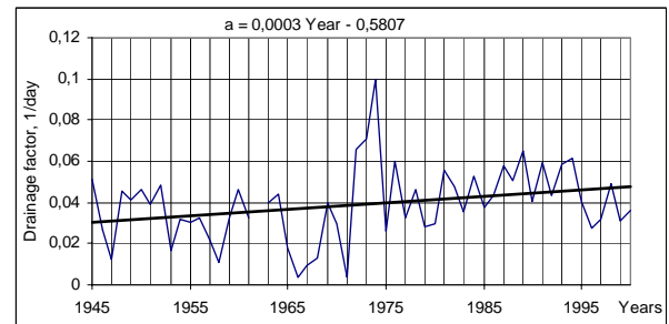
Fig. 2 Drainage factor trend of the Tuul river basin /Tuul-Ulaanbaatar/
