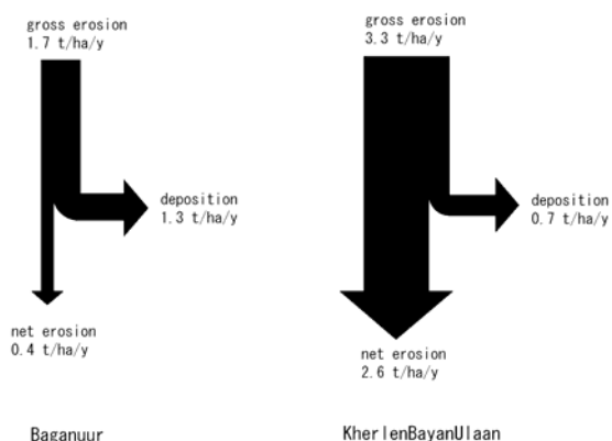
fig.2 sediment budget in the study sites
