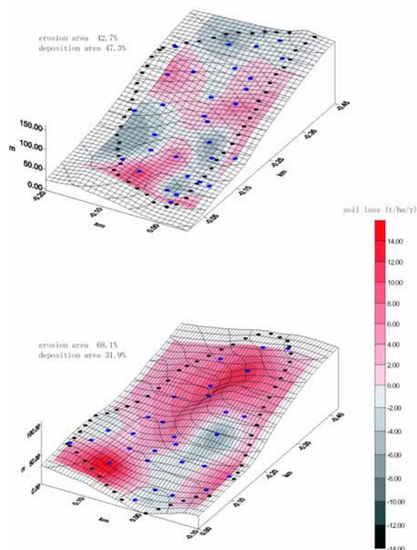
fig.1 spatial distribution of soil erosion rate
